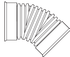
45° MITERED BEND N-12 ST AND N-12 WT
